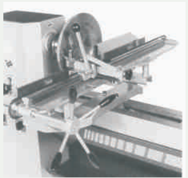
KA-90 with copying transversal support to copy plates, discs,...
